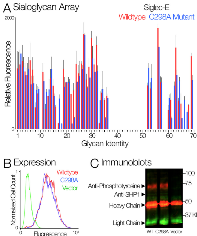
FIGURE 6. Sialoglycan array, immunoprecipitation, and Western blot with WT and mutant Siglec-E to decipher the role in ligand binding and cell signaling. A , sialoglycan arrays with WT Siglec-E-Fc and mutant (C298A) Siglec-E-Fc was performed. RFU, relative fluorescence unit. B , Siglec-E or mutant Siglec-E (C298A) was transfected in human HEK293A cells and cell surface expression was quantified using FACS. Similar expression of monomeric and dimeric Siglec-E was found on the cell surface. C , WT and mutant Siglec-E (C298A) was expressed in HEK293A cells. Siglec-E was immunoprecipitated and probed on Western blots using anti-phosphotyrosine antibody. WT and mutant Siglec-E (C298A) was expressed in HEK293A cells, Siglec-E was immunoprecipitated and probed on Western blot using SHP-1 antibody.
